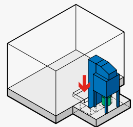
➤ Semi-automatic recovery with loading hopper with localised civil works
