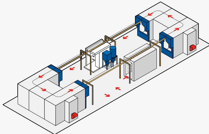
➤ Automatic powder coating system
